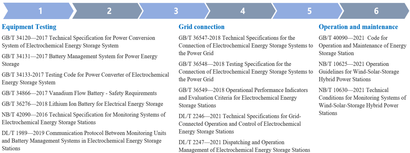
Figure 3-10 Relevant Technical Standards for Energy Storage in China
