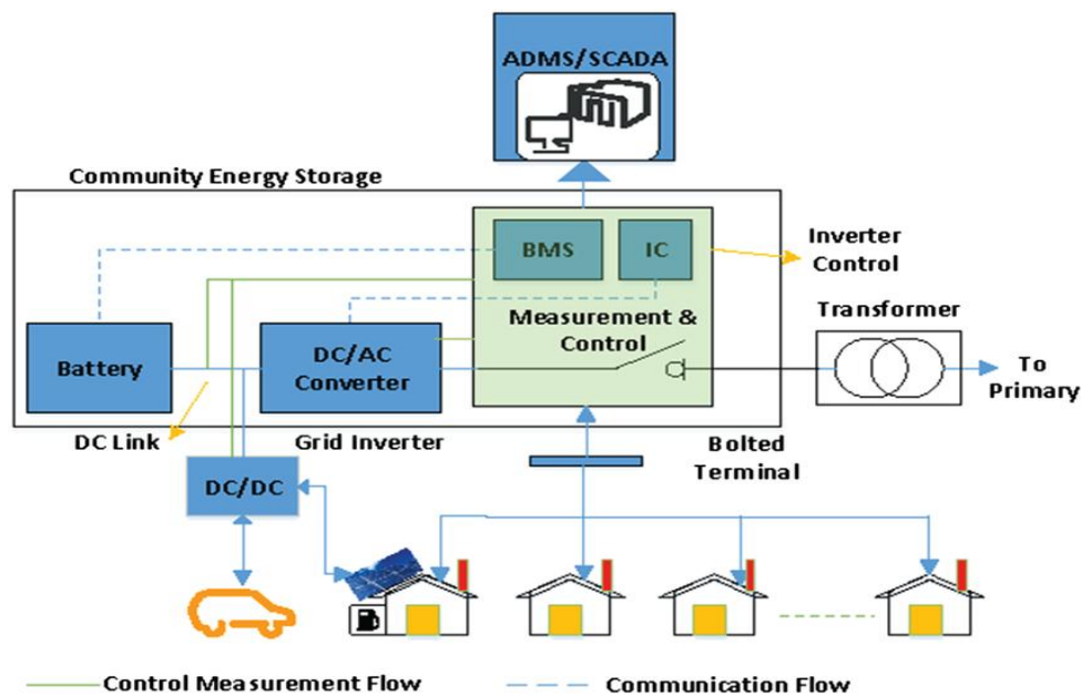
Figure 6-12 Schematic Layout of Community Energy Storage System
