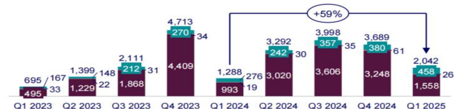
Quarterly storage deployments (MWh)
