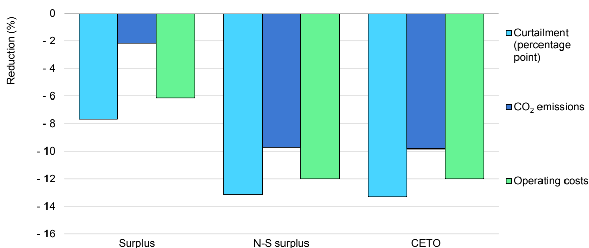
Reductions in operating costs, CO 2 emissions and curtailment under different models for regional co-ordination under current dispatching rules in China in the Announced Pledges Scenario, 2035
