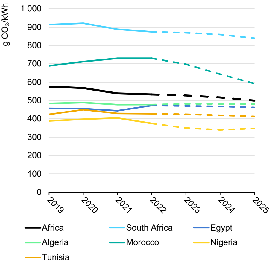
Development of average CO 2 intensity, Africa, 2019-2025
