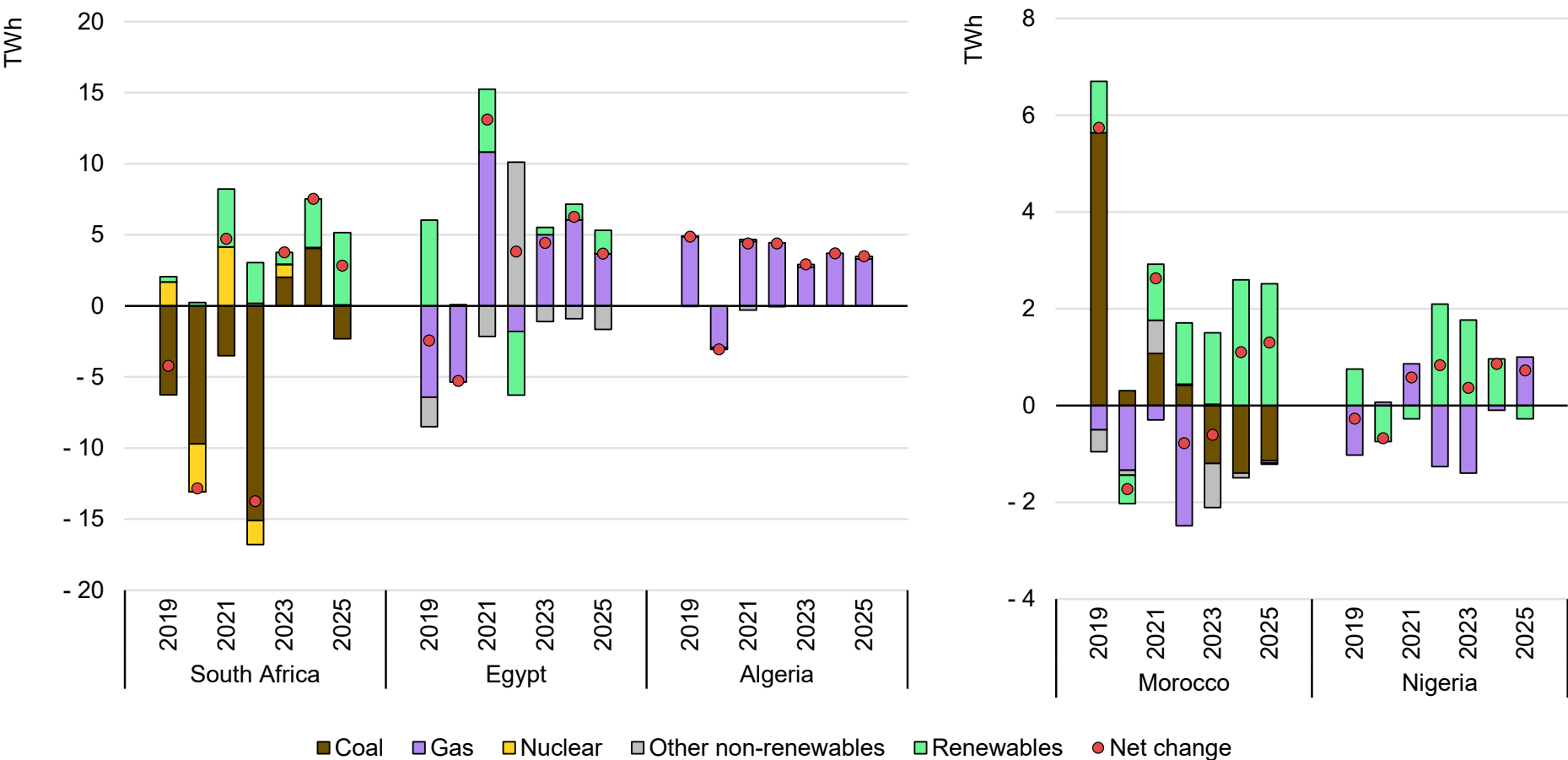
Year-on-year change in electricity generation in selected countries in Africa, 2019-2025
