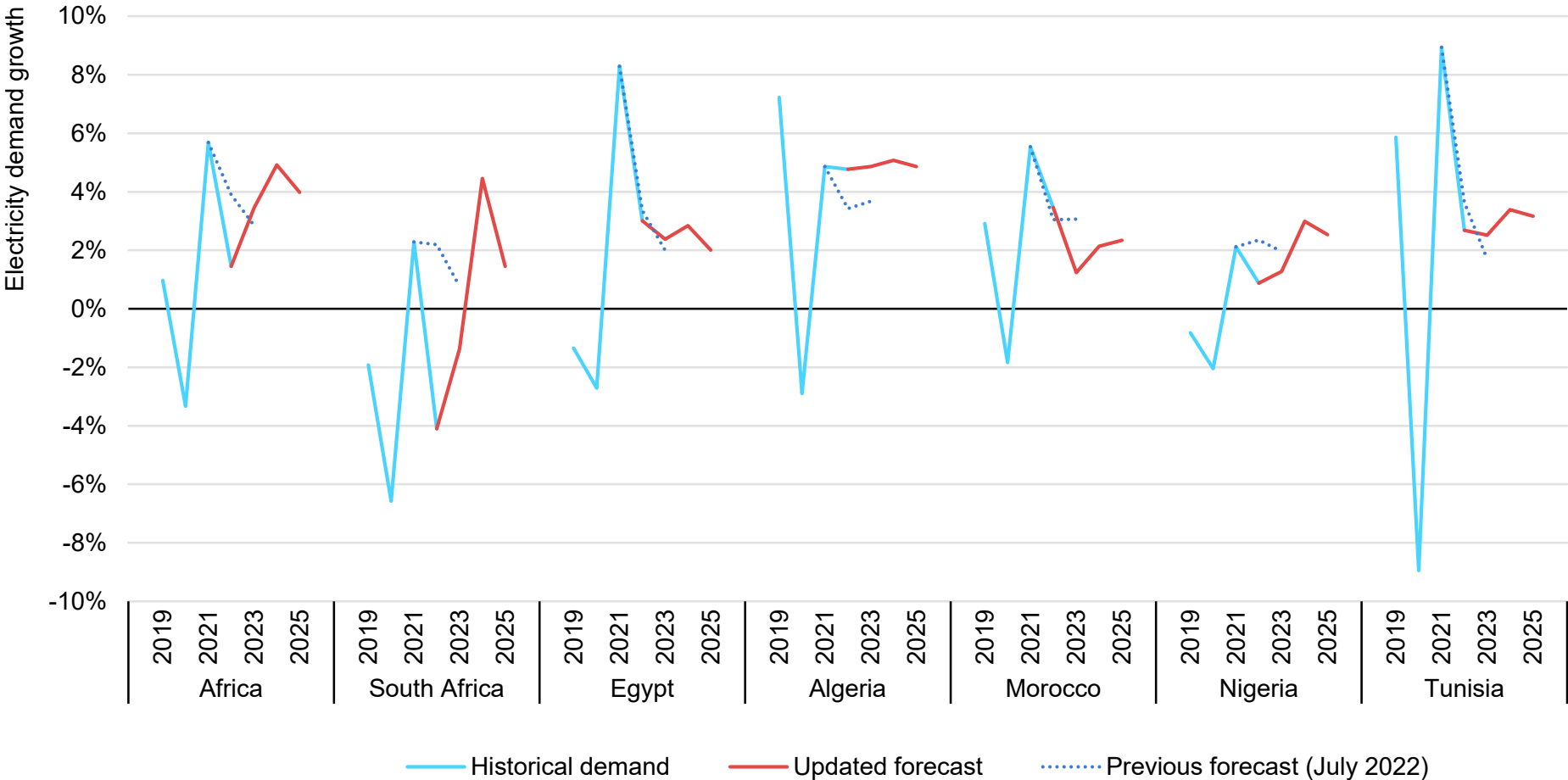
Year-on-year relative change in electricity demand, Africa, 2019-2025
