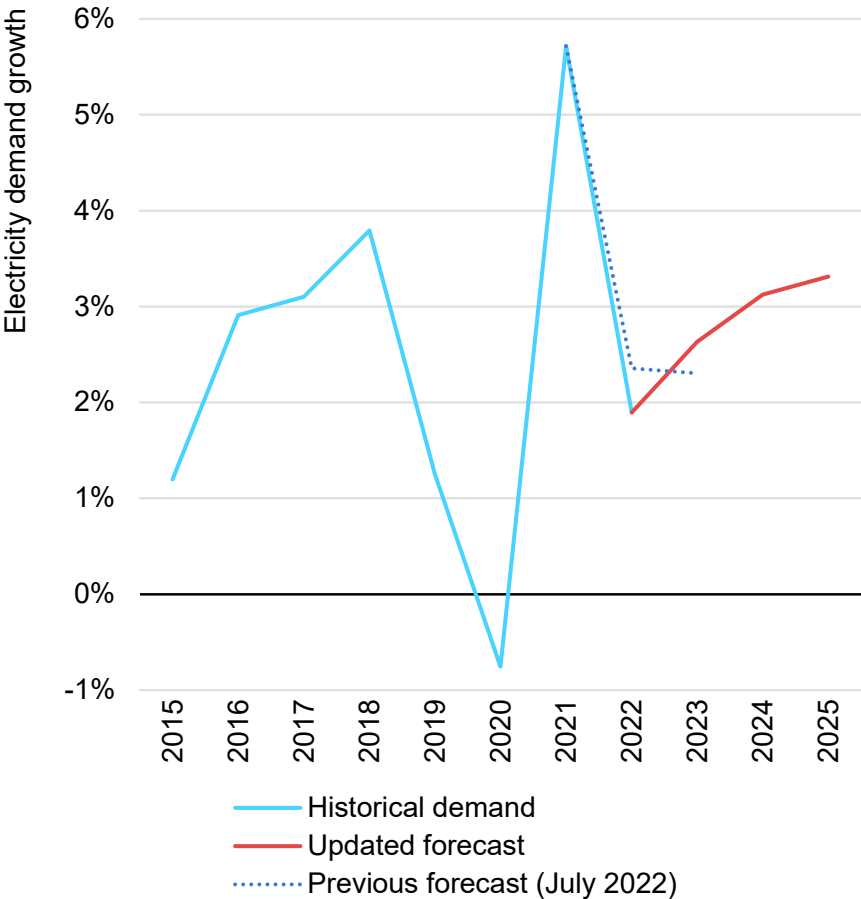
Year-on-year relative global change in electricity demand, 2015-2025
