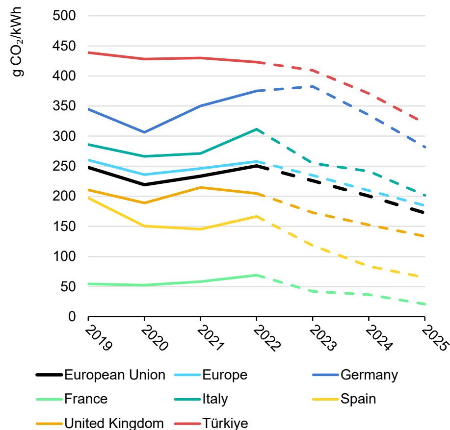
Development of average CO 2 intensity, Europe, 2019-2025
