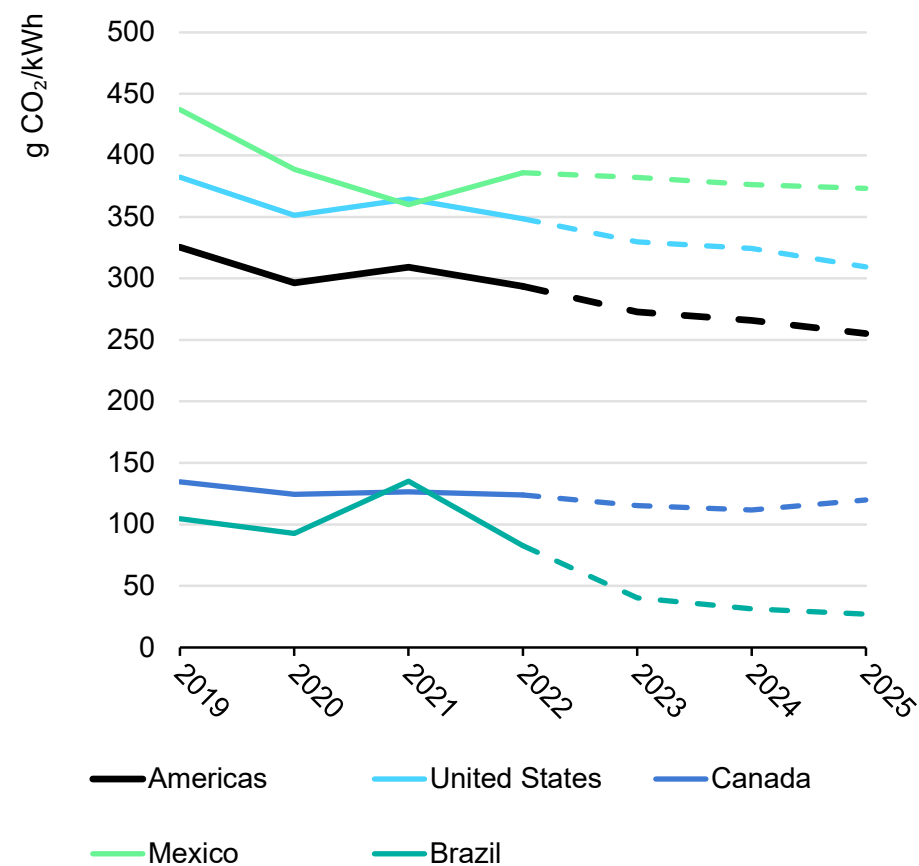
Development of average CO 2 intensity, Americas, 2019-2025
