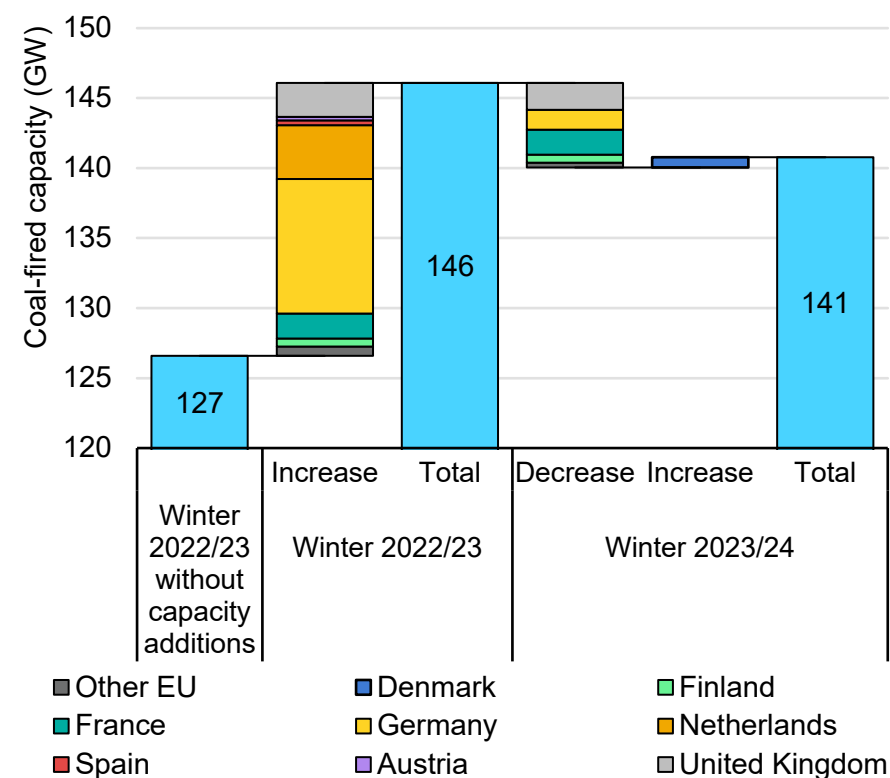
Breakdown of coal-fired capacity and capacity extensions in selected European countries, 2022-2024
