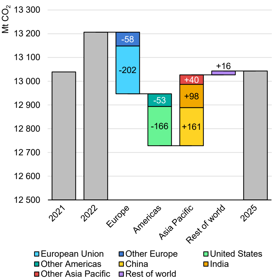
Changes in global emissions of power generation, 2021-2025
