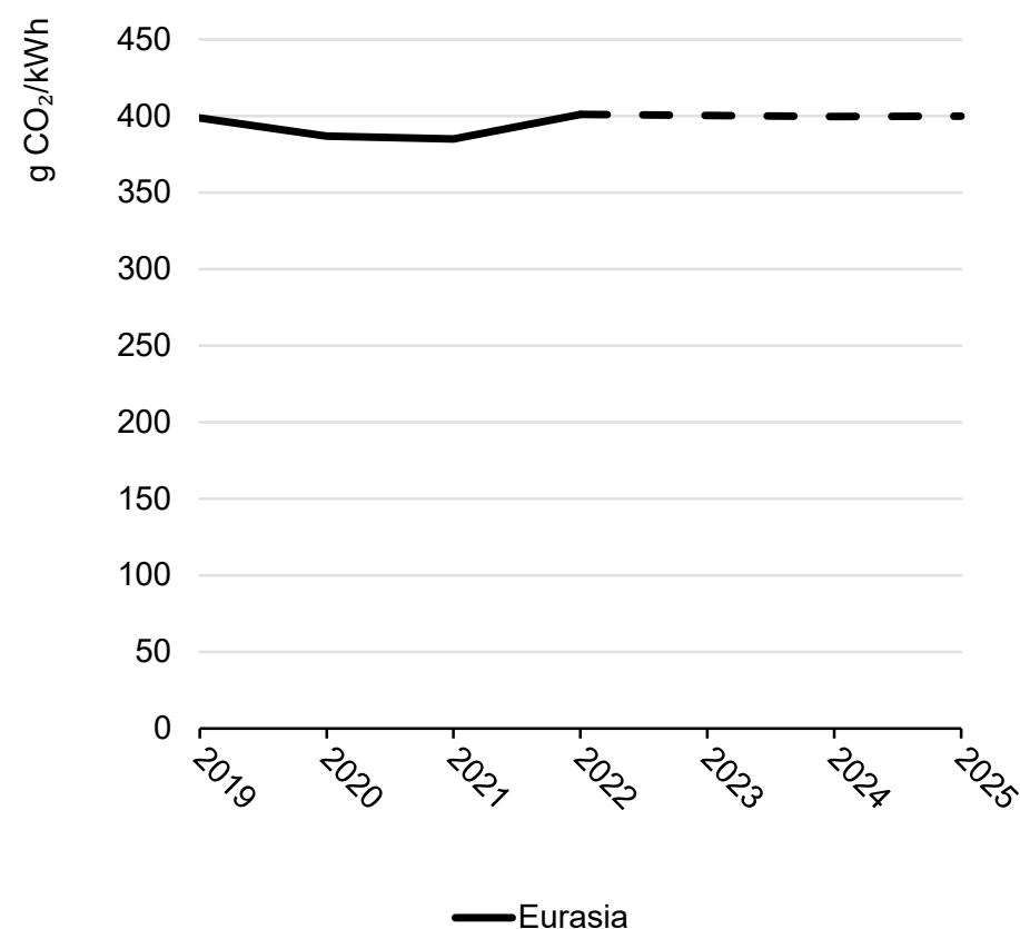
Development of average CO 2 intensity, Eurasia, 2019-2025
