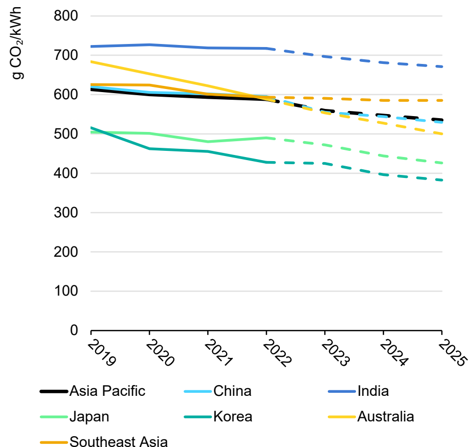
Development of average CO 2 intensity, Asia Pacific, 2019-2025
