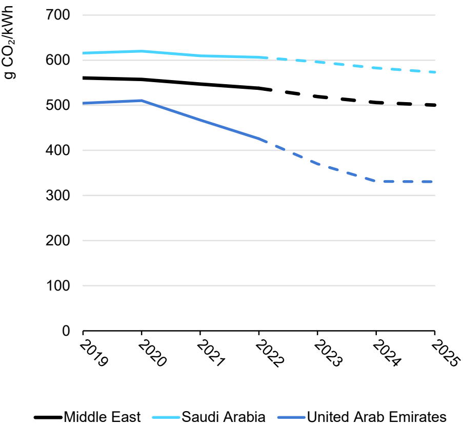
Development of average CO 2 intensity, Middle East, 2019-2025
