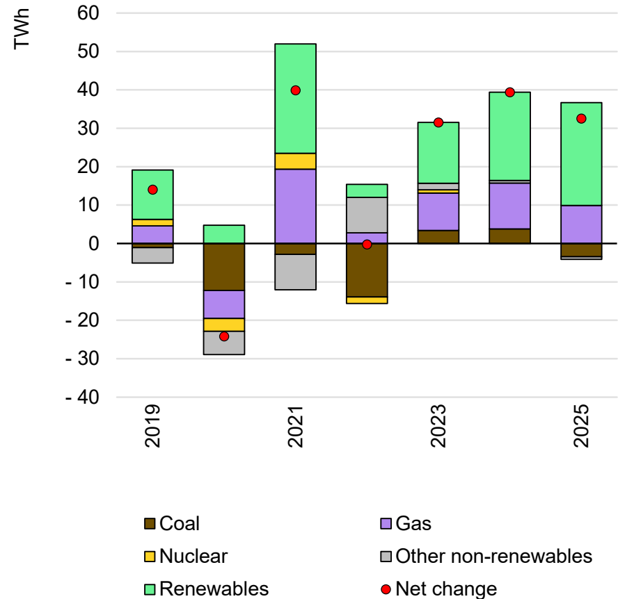
Year-on-year change in electricity generation, Africa, 2019-2025
