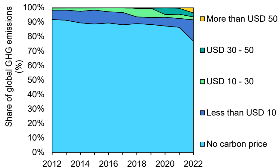
Share of global GHG emissions covered by a carbon price, by price level, 2012-2022
