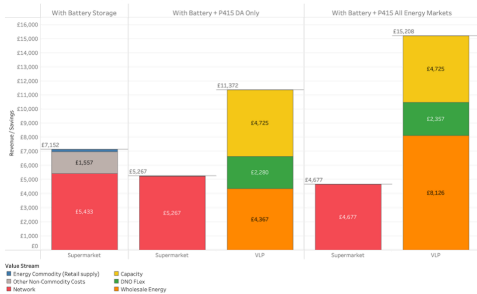
Annual Value from 500kWh/250kW Battery Storage
