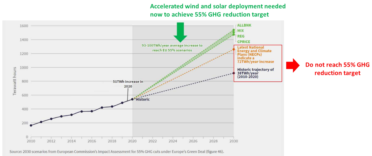
Figure 3: Wind and Solar Growth required to reach EU's 55% Emissions Target by 2030, (adapted from EMBER, Agora Energiewende, The European Power Sector in 2019)
