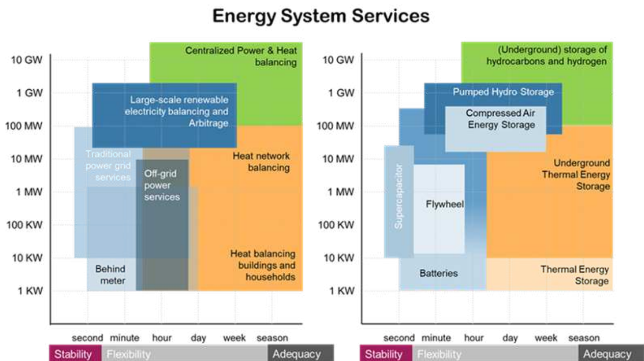
Figure 8: Energy system services and storage options mapped according to their power (W) and relevant timescales for charging and discharging. Colours coding indicate in which infrastructure system the storage technology is implemented: blue = electricity grids, green = (renewable) gas infrastructure; orange is heat networks adapted from ref [36].
