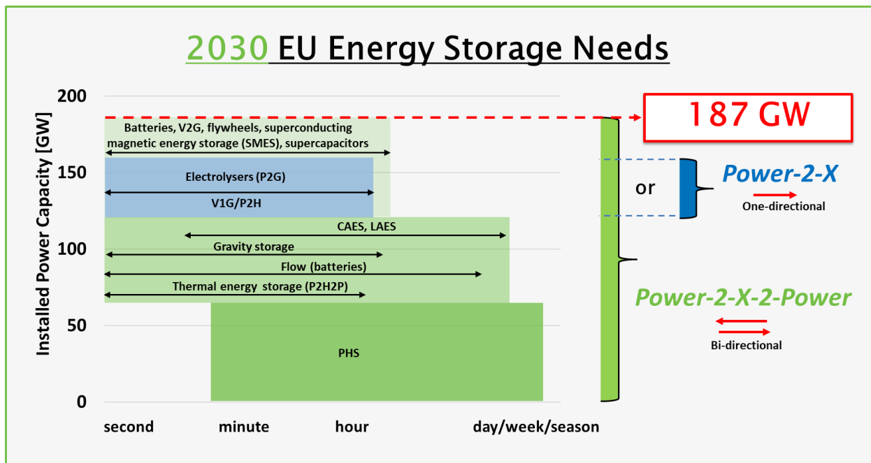
Figure 12: Total energy storage requirements by 2030. The Y-axis shows installed power capacity (GW) for different energy storage technologies based on total flexibility as defined in the EC study on energy storage values, assumptions on replacing gas turbines by 2030 and other literature studies. Power-to-X technologies are highlighted in blue and provide system flexibility in one-direction. Power-to-X-to-Power technologies are shown in green and provide system flexibility that is bi-directional i.e. electricity is given back to the system, these technologies provide critical energy shifting services. The total energy storage needs are indicated by the red dotted line and are at least 187 GW in 2030, this includes new and existing storage installations (where existing installations in Europe are approximated to be 60 GW including 57 GW PHS [43] and 3.8 GW batteries according to IEA Energy Storage 2021 report*).
