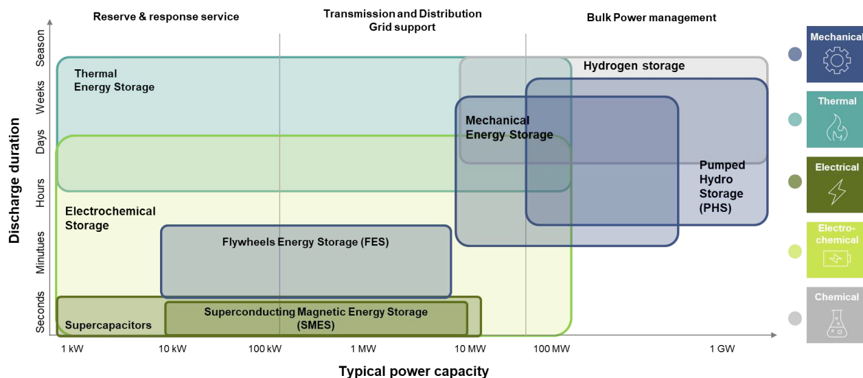
Figure 5: Typical power ranges and discharge duration of different energy storage technologies.
