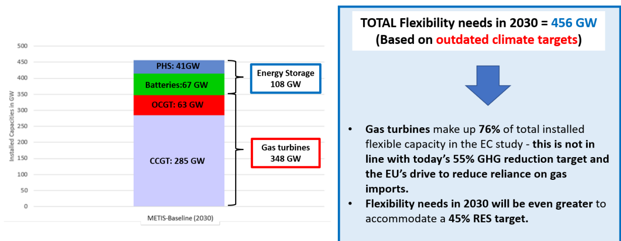
Figure 10: Installed power capacities for flexibility solutions from METIS-baseline 2030 scenario adapted from the EC Study on energy storage [20].
