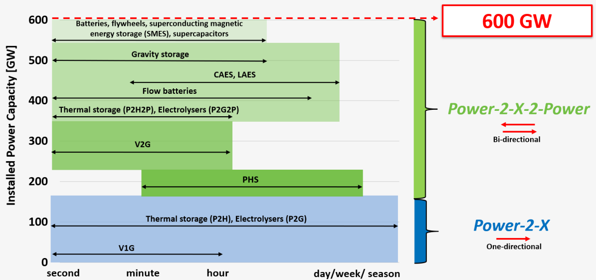
Figure 13: Total energy storage requirements by 2050. The Y-axis shows installed power capacity (GW) for different energy storage technologies based on total flexibility needs as defined in the EC study on energy storage and values from other literature studies. Power-to-X technologies are highlighted in blue and provide system flexibility in one-direction. Power-to-X-to-Power technologies are shown in green and provide system flexibility that is bi-directional i.e. electricity is given back to the system, these technologies provide critical energy shifting services. The total energy storage needs are indicated by the red dotted line to be at least 600 GW in 2050.
