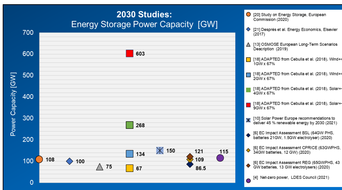
Figure 6: Energy Storage installed power capacity requirements across different literature studies for 2030 focused on Europe.
