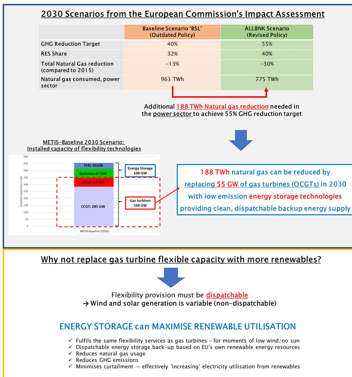
Figure 11: Overview of rationale for replacing gas turbines using natural gas for flexible backup supply with energy storage in the power sector in 2030 based on data from the EC Impact Assessment and EC study on energy storage.
