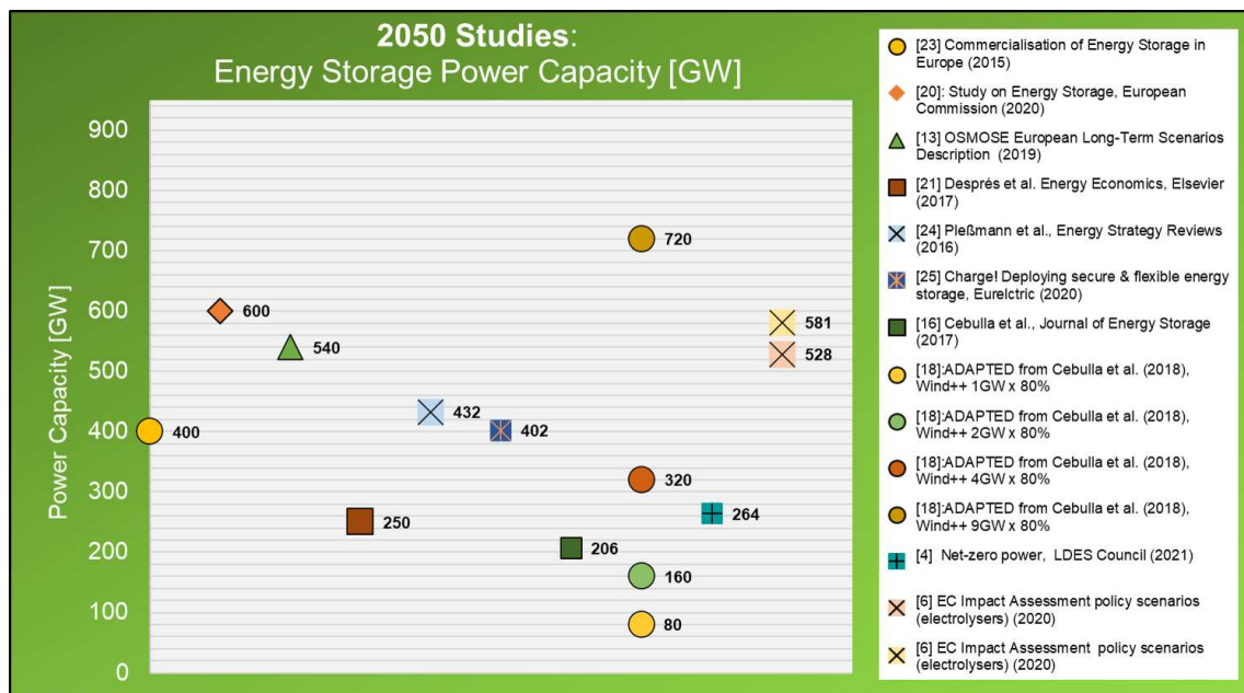
Figure 7: Energy Storage installed power capacity requirements across different literature studies for 2050 focused on Europe.
