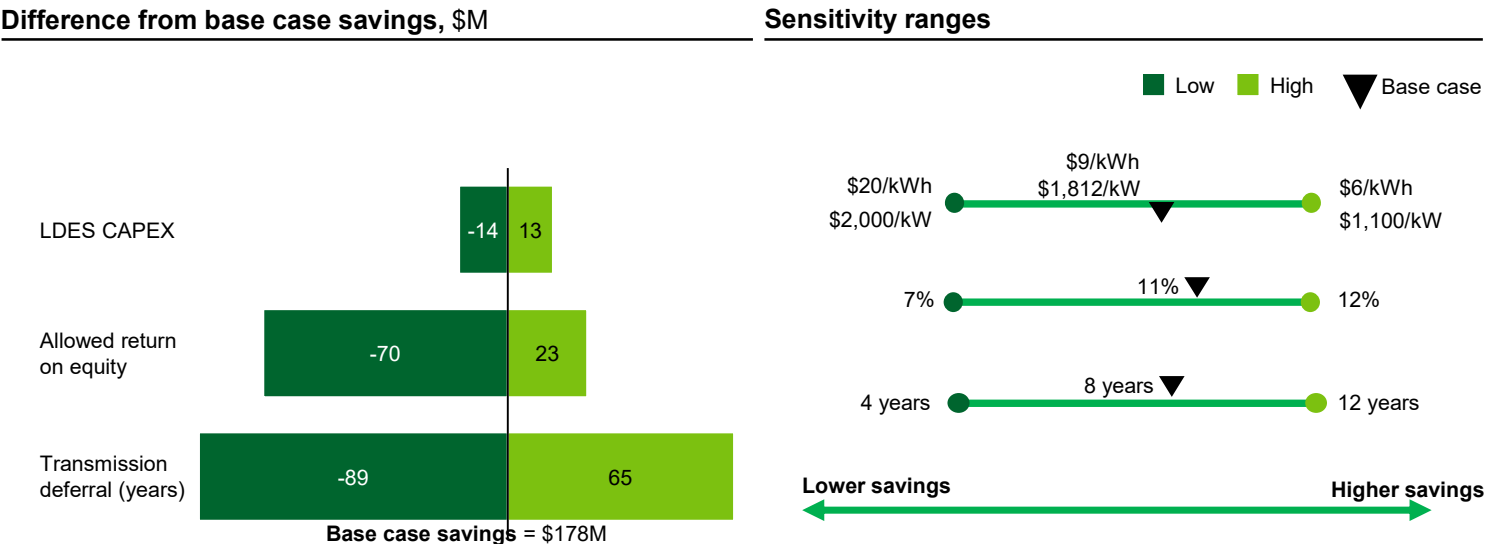
Figure 20: Even in conservative deferral sensitivities, LDES can provide an attractive financial value proposition for T&D deferral i
