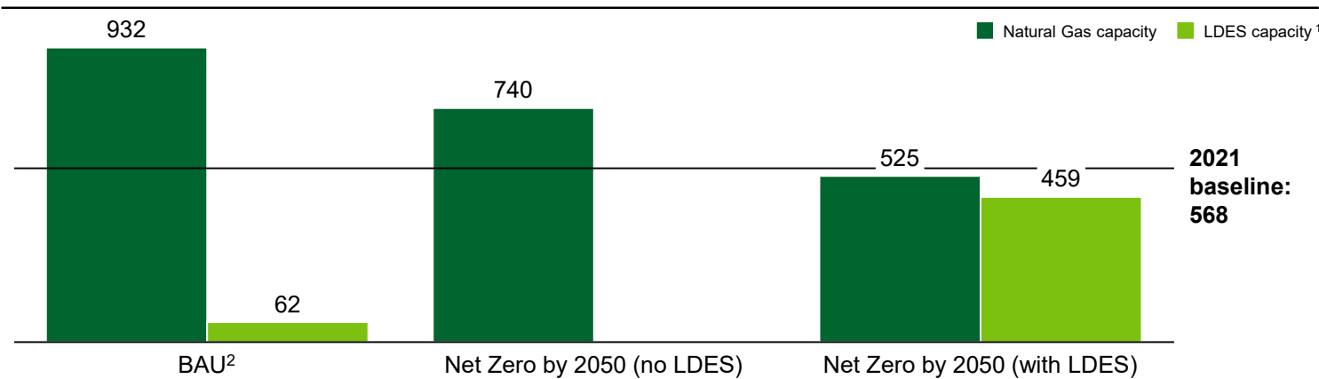
Figure 2: Under a “Net-Zero by 2050” scenario, multi-day / week LDES may supplant as much as 200+ GW of new natural gas (i.e., peaking) capacity in net-zero scenarios, dependent upon the level of gas retirements. Most Natural Gas capacity in the Net Zero scenarios is due to existing natural gas, which remains on the system. In no-LDES scenarios, net new systems are built. i 1 Includes both Diurnal and Seasonal LDES but does not include Li-ion; 2 BAU stands for Business as Usual.
