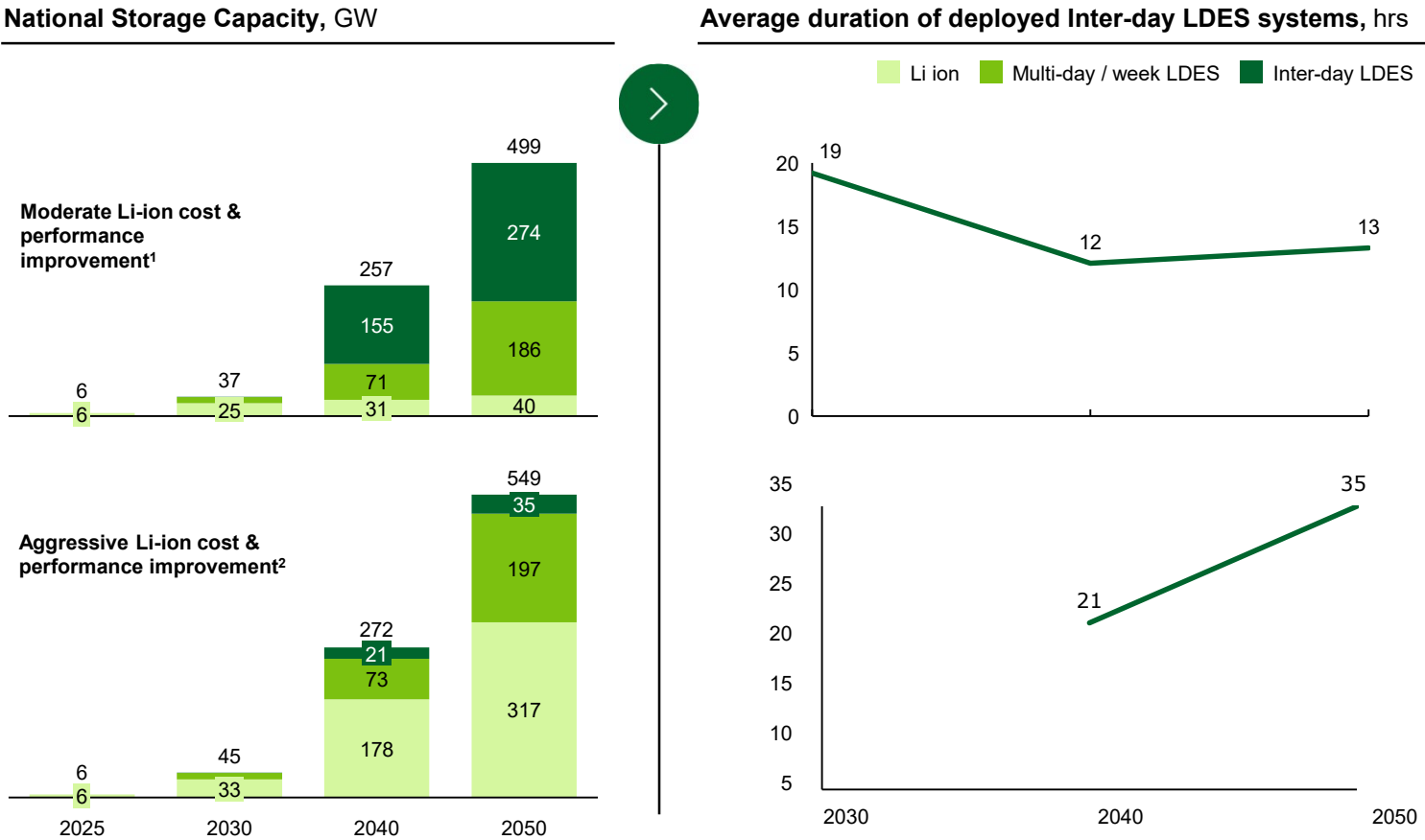
Figure 7: Deployments of inter-day LDES technologies depend on whether they can outcompete Li-ion’s cost and performance. xii Average duration of Inter-day LDES systems is lowered if Li-ion costs are in-line with predictions since more ~10-hour LDES systems will come online. However, if Li-ion costs reduce aggressively, Li-ion will be built instead of 10-hour LDES systems, and economic LDES systems will be longer duration (20+hour). No duration is shown for 2030 in the aggressive Li-ion scenario due to limited projected Inter-day LDES deployment. 1 Assumes Li-ion batteries improve costs and performance at a moderate rate based on current Li-ion cost curves (54% cost improvements through 2030 and 65% total improvements through 2050 relative to 2021 prices); 2 Assumes capex costs associated with energy component (i.e., battery cell) are 50% lower than in moderate scenario.
