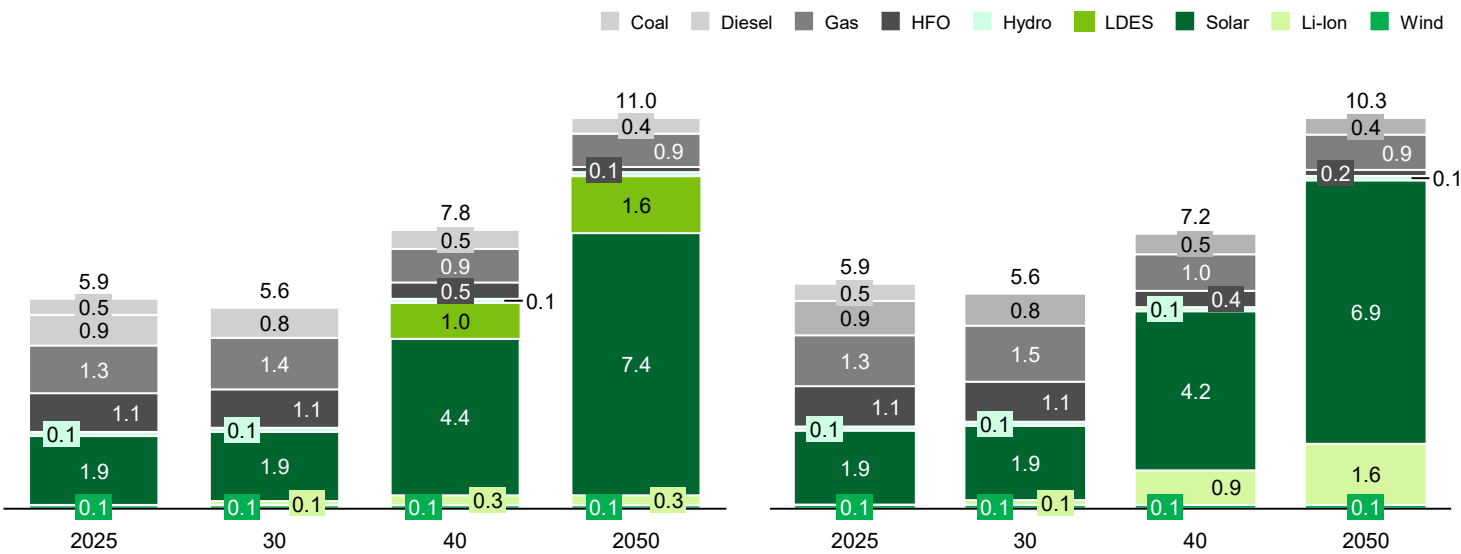
Figure 21: The modeled generation transition in the “net-zero by 2050” scenario for Puerto Rico identifies a potential need for 1.6 GW of LDES as a part of a “least-cost” pathway. i
