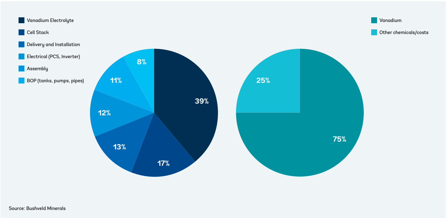
Figure 2.6: VRFB Cost Breakdown
