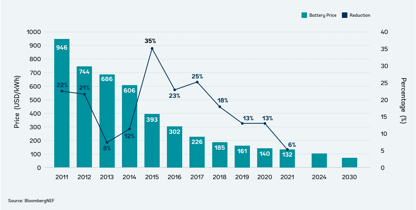
Figure 2.5: Lithium-ion Battery Cost Trajectory
