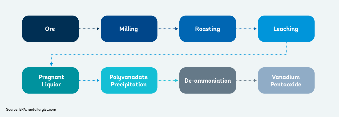
Figure 3.1: Steps for Processing Vanadium Ore to Vanadium Salts
