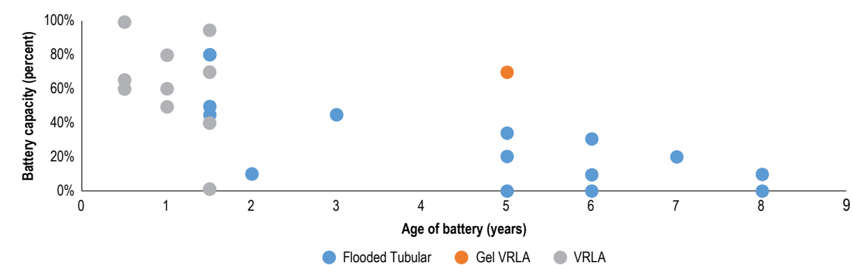
FIGURE B.1: Capacity of Flooded Tubular, Valve Regulated Lead Acid (VRLA), and VRLA Gel Batteries in First Eight Years
