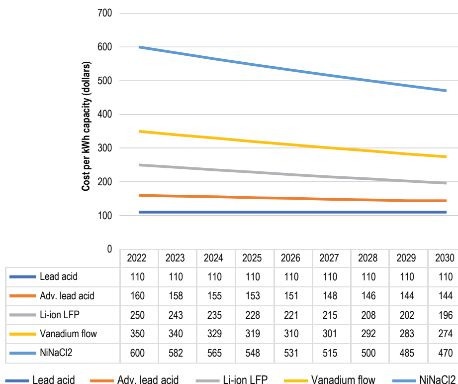
FIGURE 3.2: Cost of Six-Hour Storage, by Battery Type, 2022–30
